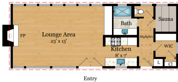
GUEST HOUSE ABOVE STORAGE 680 SQ FT
